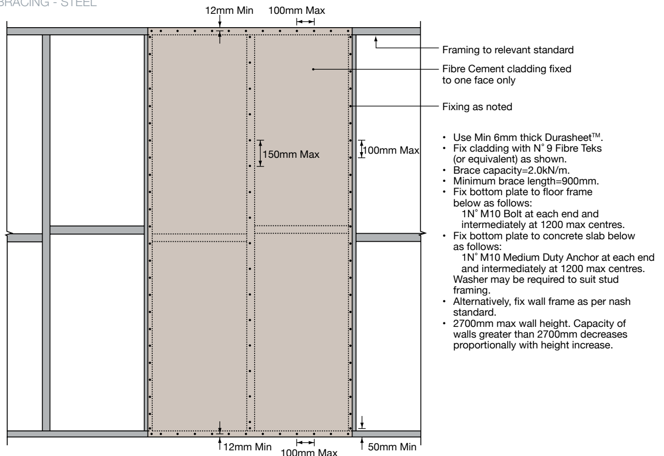
FIGURE 12 // TYPE A BRACING - STEEL
