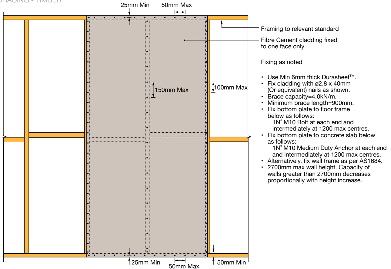
FIGURE 13 // TYPE B BRACING - TIMBER
