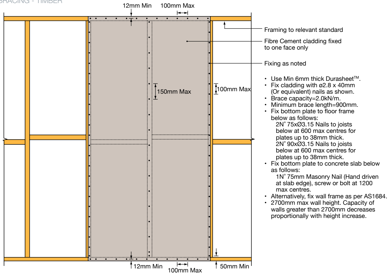
FIGURE 11 // TYPE A BRACING - TIMBER
