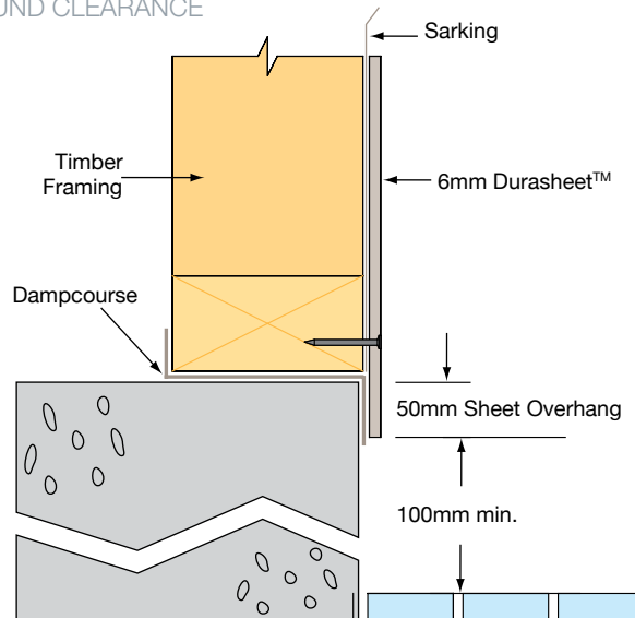
FIGURE 10 // GROUND CLEARANCE
