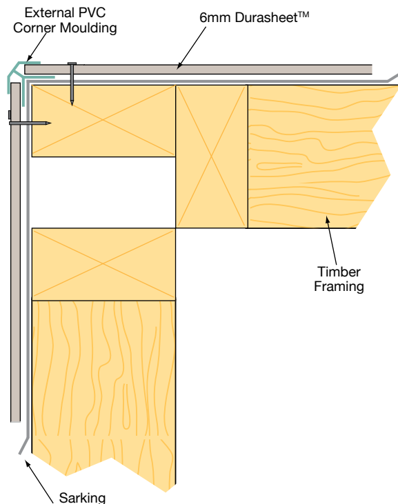
FIGURE 9 // EXTERNAL CORNERS PVC SHEET JOINERS
