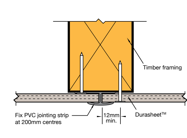
FIGURE 2 // GARAGE / CARPORT / ALFRESCO LININGS
