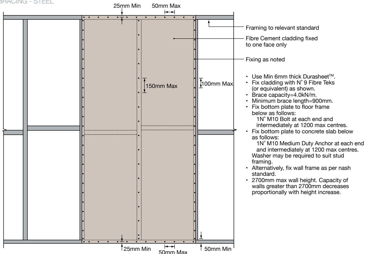
FIGURE 14 // TYPE B BRACING - STEEL
