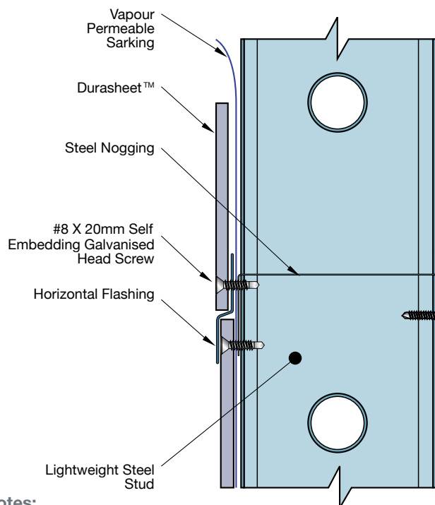
FIGURE 5 // HORIZONTAL JOINT DETAIL
