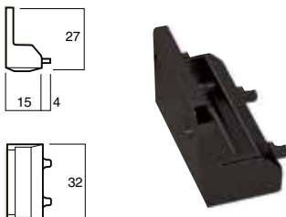
Timber frame strike
