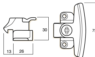
Lockable
