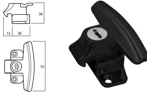
Lockable body
