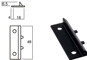
16 mm flat strike
