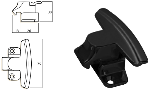
Non-lockable body
