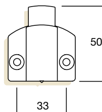
Unlocked Position
