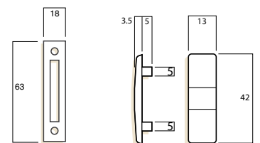
Flat keeper
